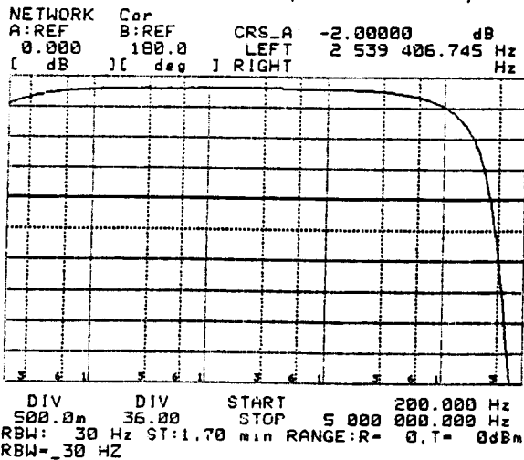
040-0080 Insertion Loss(2 Units Back to Back)
