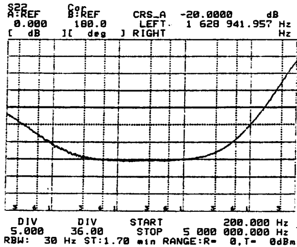
040-0080 50-600 Ohm Return Loss
