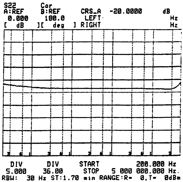
040-0084 50-135 Ohm Return Loss
