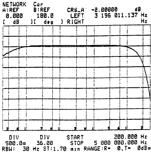
040-0084 Insertion Loss(2 Units Back to Back)
