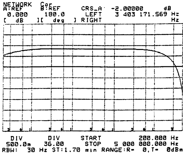
040-0088 Insertion Loss(2 Units Back to Back)
